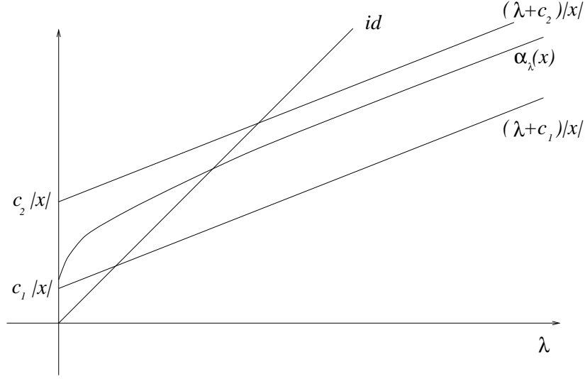
FIGURE 1. \alpha_\lambda(x) in dependence of \lambda
