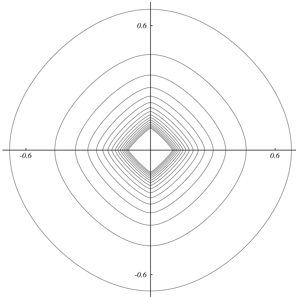
FIGURE 2. The unit sphere of \alpha in two dimensions for the constant potentials \lambda = \frac{1}{2}, 1, \frac{3}{2}, 2, \dots, 8 (from outside inwards)
